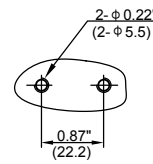
Rear bracket mounting
